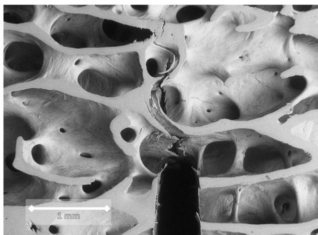
Fig. 1. Crack growth emanating from the man-made notch as in the SENB FT tests of Cook and Zioupos (2009) and Ding and Hvid (2000). Following application of bending moments on either side the notch opens up and the trabeculae ahead of it start snapping. The deformation and crack growth was stopped as soon as this first critical load was reached. The load was used to define the K_{\text{IC}} value (initial notch width \sim 300 \mu\text{m} ).
