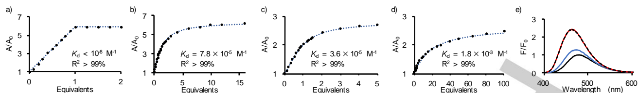
Figure 5. UV-vis ( \lambda = 322 nm) titrations of 7 (100 \mu M) with M(ClO_4)_2 as a function of a) Zn^{2+} , b) Zn^{2+} (2% H_2O -MeCN), c) Cd^{2+} (MeCN), d) Cd^{2+} (2% H_2O -MeCN). e) Emission spectrum ( \lambda_{ex} = 380 nm) of 7 in 2% H_2O -MeCN (black), + 5 equiv. Cd^{2+} (blue), + 5 equiv. Zn^{2+} (red), + 5 equiv. each Zn^{2+} and Cd^{2+} (black dashed).
