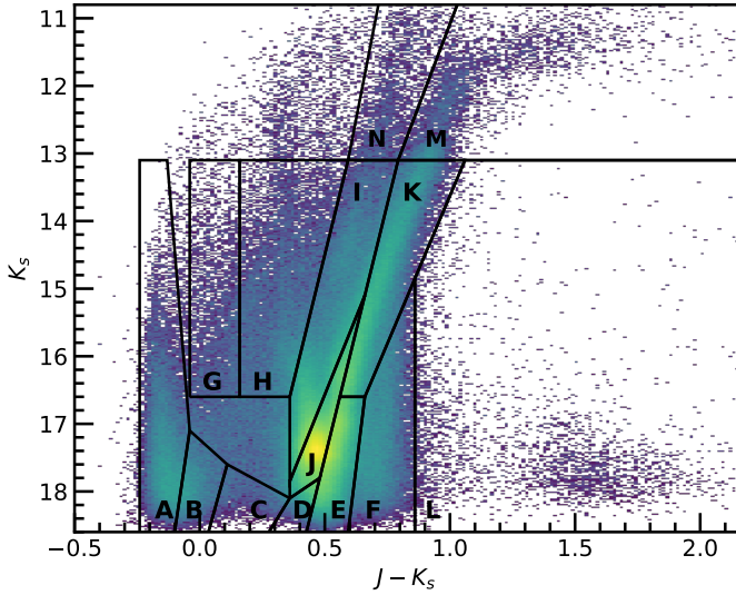
Fig. 1. Stellar density (Hess) diagram in the (J - K_s, K_s) color-magnitude space of all sources with proper motions measurements. Overplotted as black polygons are regions of different stellar populations as defined by Cioni et al. (2016) and El Youssoufi et al. (in prep.), the latter adding regions M and N and extending regions A and L.
