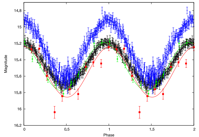
Figure 5. [3.6] (black +), [4.5] (blue circles), [5.8] (green diamonds) and [8.0] (red squares) \mu\text{m} light curves of WD0137–349 folded on the ephemeris of the system.
