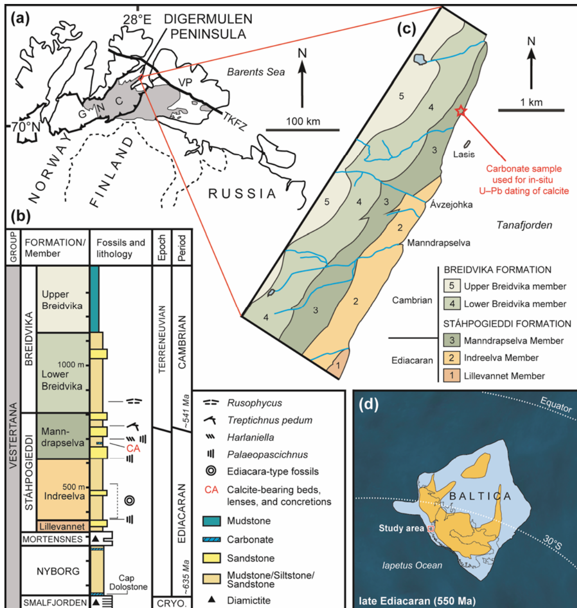
Fig. 1. (Colour online) (a) Outline of northernmost Scandinavia showing the Vestertana Group rocks, in grey shade, preserved within the Gaissa Nappe Complex (GNC) and parautochthonous in eastern Finnmark on the Varanger Peninsula (VP). Red box highlights the study area. TKFZ – Trollfjorden–Komagelva Fault Zone. (b) Simplified stratigraphy of the Vestertana Group (after Jensen et al. 2018b), showing occurrences of carbonates in the Ediacaran strata in eastern Finnmark. The stratigraphic position of carbonates, some with calcite spherulites and CIC calcite, analysed in the study are indicated 'CA'. (c) Geology of the SE portion of the Digermulen Peninsula, based on Siedlecka et al. (2006), showing locality where carbonates were found within the Mann-drapselva Member. We refer to Meinhold et al. (2019a) for details. (d) Late Ediacaran (550 Ma) palaeogeographic reconstruction of Baltica (after Meert, 2014). Land (ochre) and shallow sea (light blue) distributions were adopted from the palaeogeographic map series of Ron Blakey (Global Paleogeography and Tectonics in Deep Time ©2016 Colorado Plateau Geosystems Inc., used under an Academic Content License Agreement). Red box highlights the study area.
