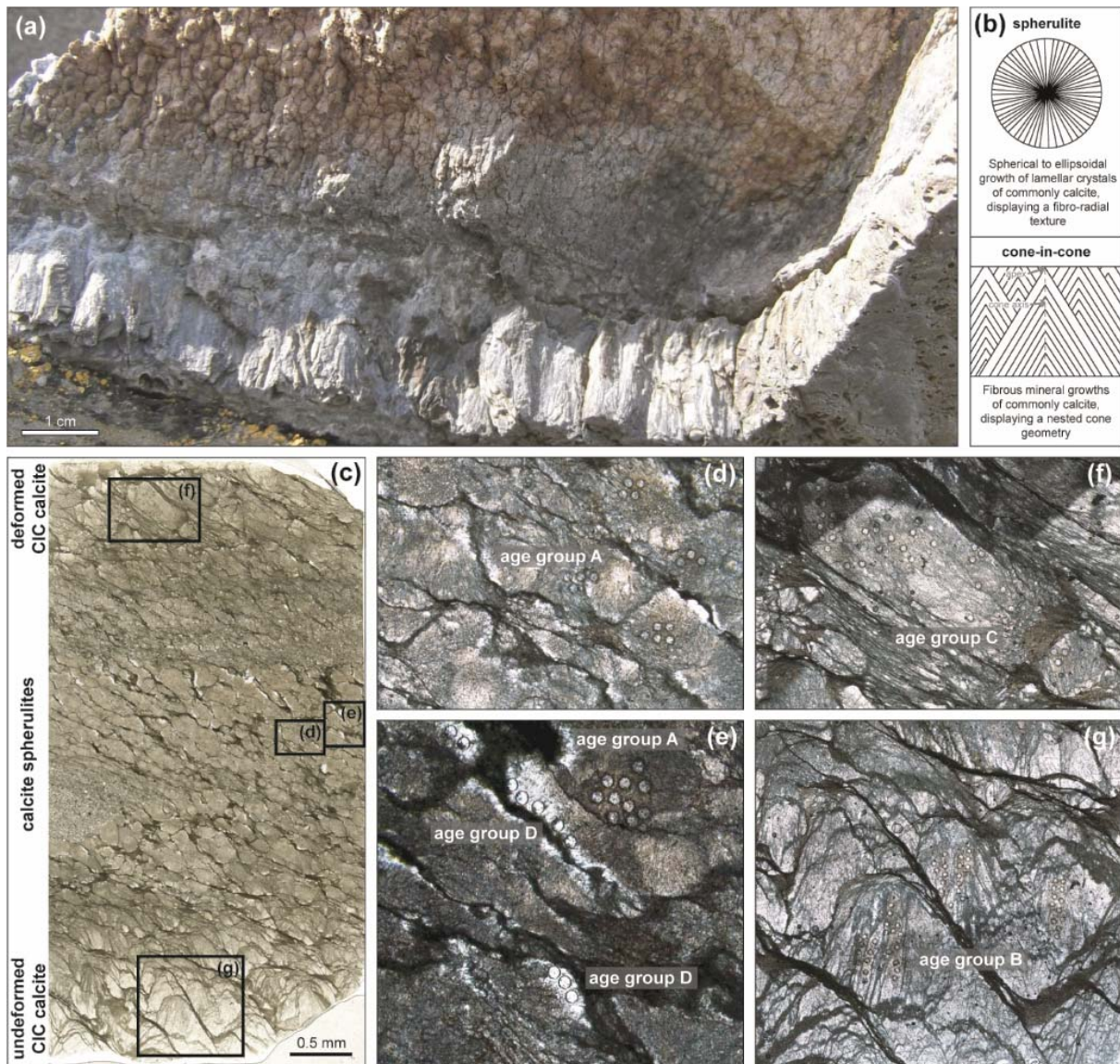
Fig. 2. (Colour online) (a) Field photograph showing calcite spherulites and undeformed CIC calcite from the second cycle of the Manndrapselva Member of the Stáhpogieddi Formation from the eastern part of the Digermulen Peninsula, Finnmark, Arctic Norway. (b) Schematic illustrations of calcite spherulite and CIC structures (after Meinhold et al. 2019a). (c–g) Images of the thick section from sample D17-GM4 used for in situ U–Pb dating of calcite. All images oriented with top up. (c) Entire thick section. Total length of the glass slide is 4.8 cm. The outer layer (top and bottom) consists of nested cones of fibrous calcite (CIC structures). The inner layers show thinly laminated calcareous siliciclastics and calcite spherulites. CIC structures of the bottom layer are undeformed whereas CIC structures of the top layer are deformed. Detailed descriptions are given in Meinhold et al. (2019a). Representative parts of the thick section studied by U–Pb geochronology are outlined with black frames. (d) Photomicrograph showing calcite spherulites with analysed spots (age group A). (e) Calcite spherulites with analysed spots (age group A) and calcite fibres grown in small fissures alongside the spherulite rims with analysed spots (age group D). (f) CIC structures of calcite from the outer layer (top) with analysed spots (age group C). (g) CIC structures of calcite from the outer layer (bottom) with analysed spots (age group B).
