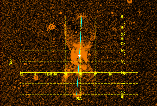
Figure 1. H\alpha continuum-subtracted image of CK Vul observed on 2010 June 22 with the Gemini North Telescope (image kindly provided by M. Hajduk). The position of the compact radio source is indicated by the white dot. The slit (cyan line) was centered on this source and passes through the tips of the ansae located near the top and bottom center of the image.
