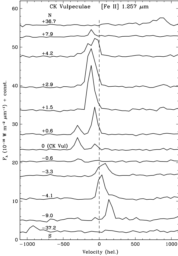
Figure 2. Spectra of the [Fe II] 1.257 \mu\text{m} line in the CK Vul nebula at the twelve locations along the slit where the line was detected. See Table 1 for details.
